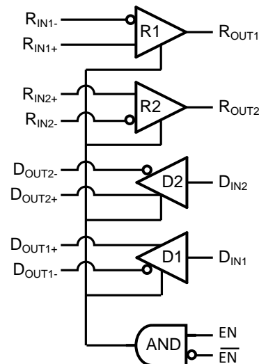
Functional Diagram
