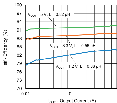
Fig. 19 - SiC437 Efficiency vs. Output Current (V_{IN} = 12\text{ V}, f_{sw} = 1\text{ MHz}, \text{ Light Load})
