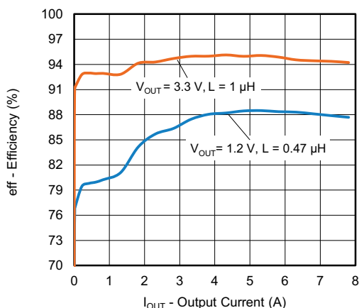
Fig. 28 - SiC438 Efficiency vs. Output Current (V_{IN} = 12\text{ V}, f_{sw} = 1\text{ MHz}, \text{ Full Load})
