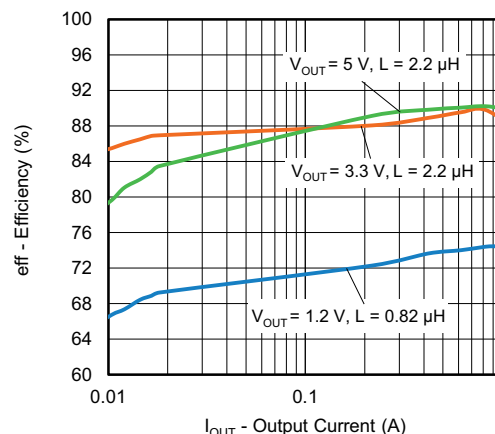
Fig. 33 - SiC438 Efficiency vs. Output Current (V_{IN} = 24\text{ V}, f_{sw} = 500\text{ kHz}, \text{ Light Load})
