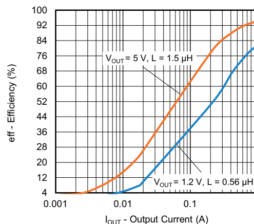
Fig. 20 - SiC437 Efficiency vs. Output Current (V_{IN} = 12\text{ V}, f_{sw} = 500\text{ kHz}, \text{ FCCM}, \text{ Light Load})
