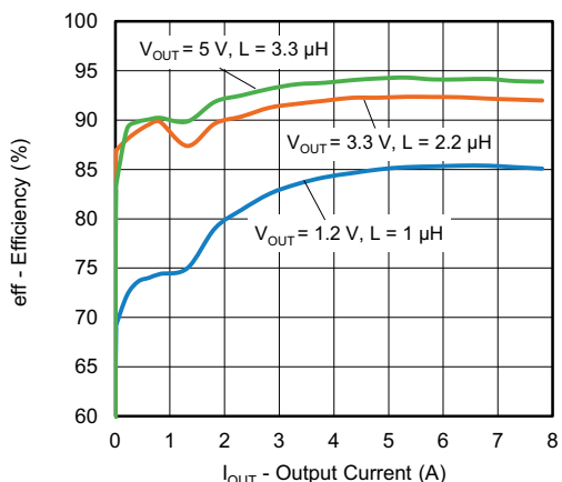
Fig. 30 - SiC438 Efficiency vs. Output Current (V_{IN} = 24\text{ V}, f_{sw} = 500\text{ kHz}, \text{ Full Load})
