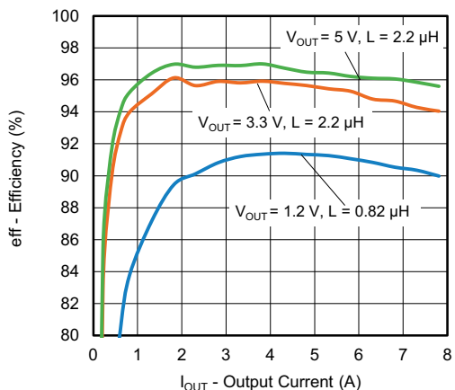
Fig. 29 - SiC438 Efficiency vs. Output Current (V_{IN} = 12\text{ V}, f_{sw} = 500\text{ kHz}, \text{ FCCM}, \text{ Full Load})
