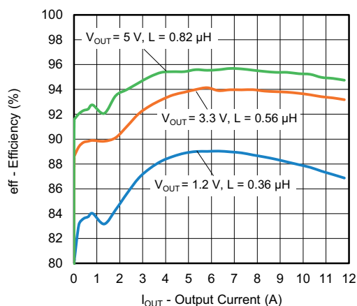
Fig. 16 - SiC437 Efficiency vs. Output Current (V_{IN} = 12\text{ V}, f_{sw} = 1\text{ MHz}, \text{ Full Load})
