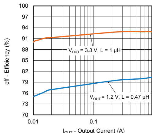
Fig. 31 - SiC438 Efficiency vs. Output Current (V_{IN} = 12\text{ V}, f_{sw} = 1\text{ MHz}, \text{ Light Load})
