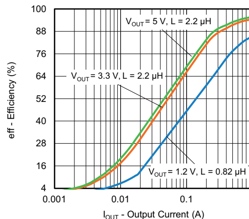
Fig. 32 - SiC438 Efficiency vs. Output Current (V_{IN} = 12\text{ V}, f_{sw} = 500\text{ kHz}, \text{ FCCM}, \text{ Light Load})
