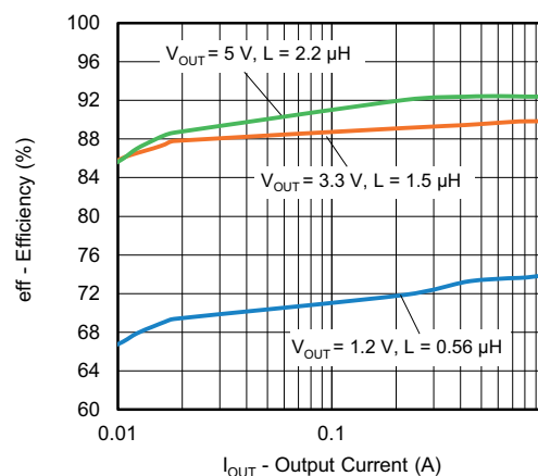
Fig. 21 - SiC437 Efficiency vs. Output Current (V_{IN} = 24\text{ V}, f_{sw} = 500\text{ kHz}, \text{ Light Load})
