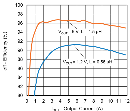
Fig. 17 - SiC437 Efficiency vs. Output Current (V_{IN} = 12\text{ V}, f_{sw} = 500\text{ kHz}, \text{ FCCM}, \text{ Full Load})
