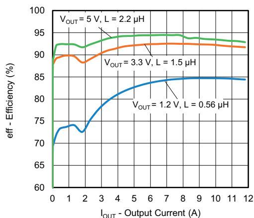
Fig. 18 - SiC437 Efficiency vs. Output Current (V_{IN} = 24\text{ V}, f_{sw} = 500\text{ kHz}, \text{ Full Load})
