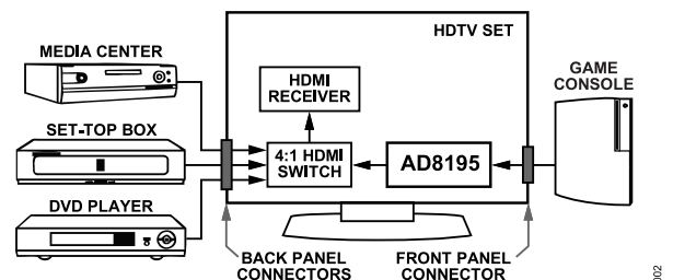
Figure 2. Typical AD8195 Application for HDTV Sets
