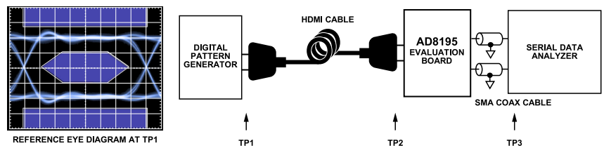
Figure 4. Test Circuit Diagram for Rx Eye Diagrams
