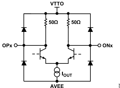
Figure 31. High Speed Output Simplified Schematic
