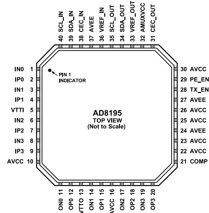
Figure 3. Pin Configuration
