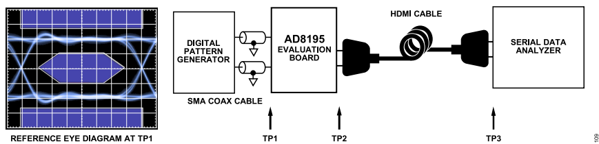
Figure 13. Test Circuit Diagram for Tx Eye Diagrams
