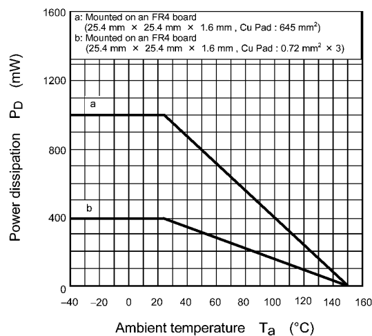
Fig. 8.15 P_D - T_a
