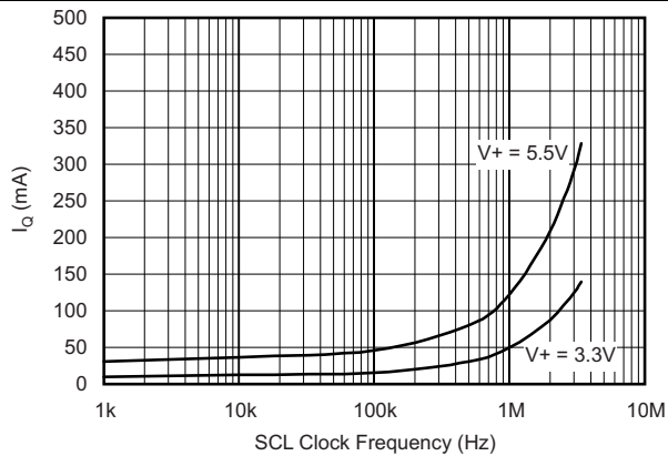
Figure 5. Shutdown Quiescent Current vs SCL Clock Frequency
