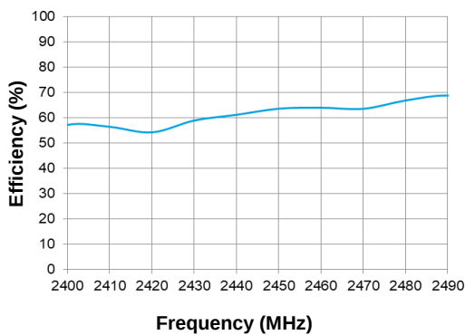
2.4 GHz Efficiency
