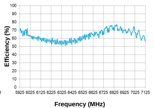
6 / 7 GHz Efficiency
