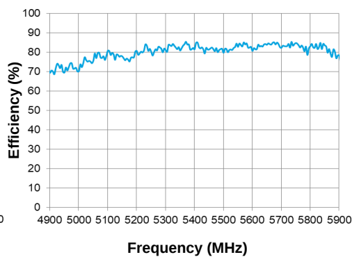
5 GHz Efficiency
