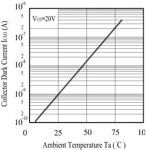
Fig.5 Collector Dark Current vs. Ambient Temperature
