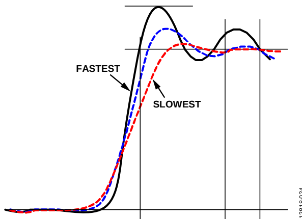
Figure 22. Switching Node at Various Slew Rate Settings
