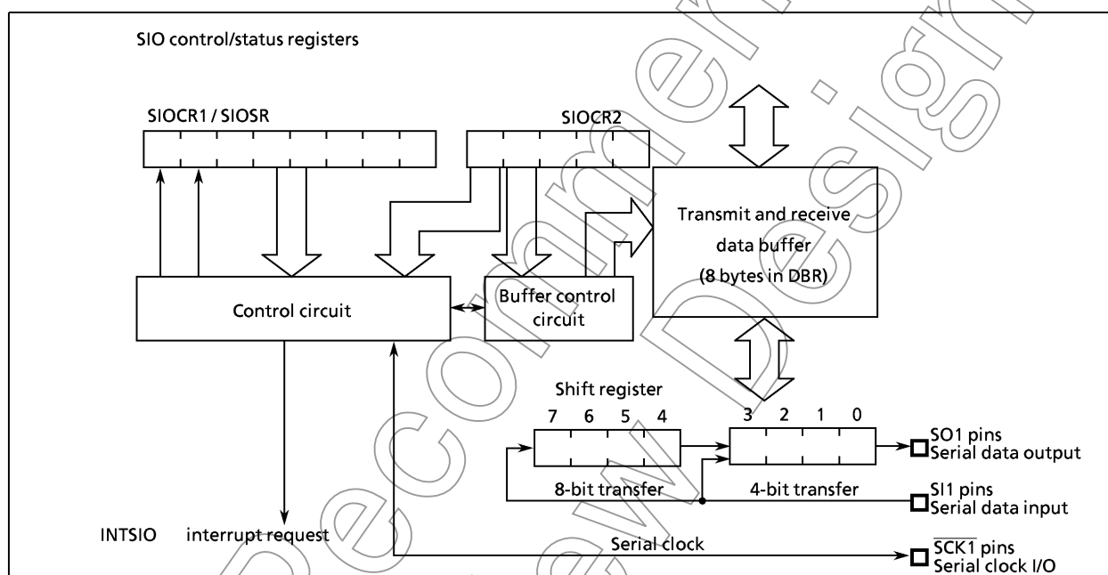
Figure 2-31. Serial Interfaces
