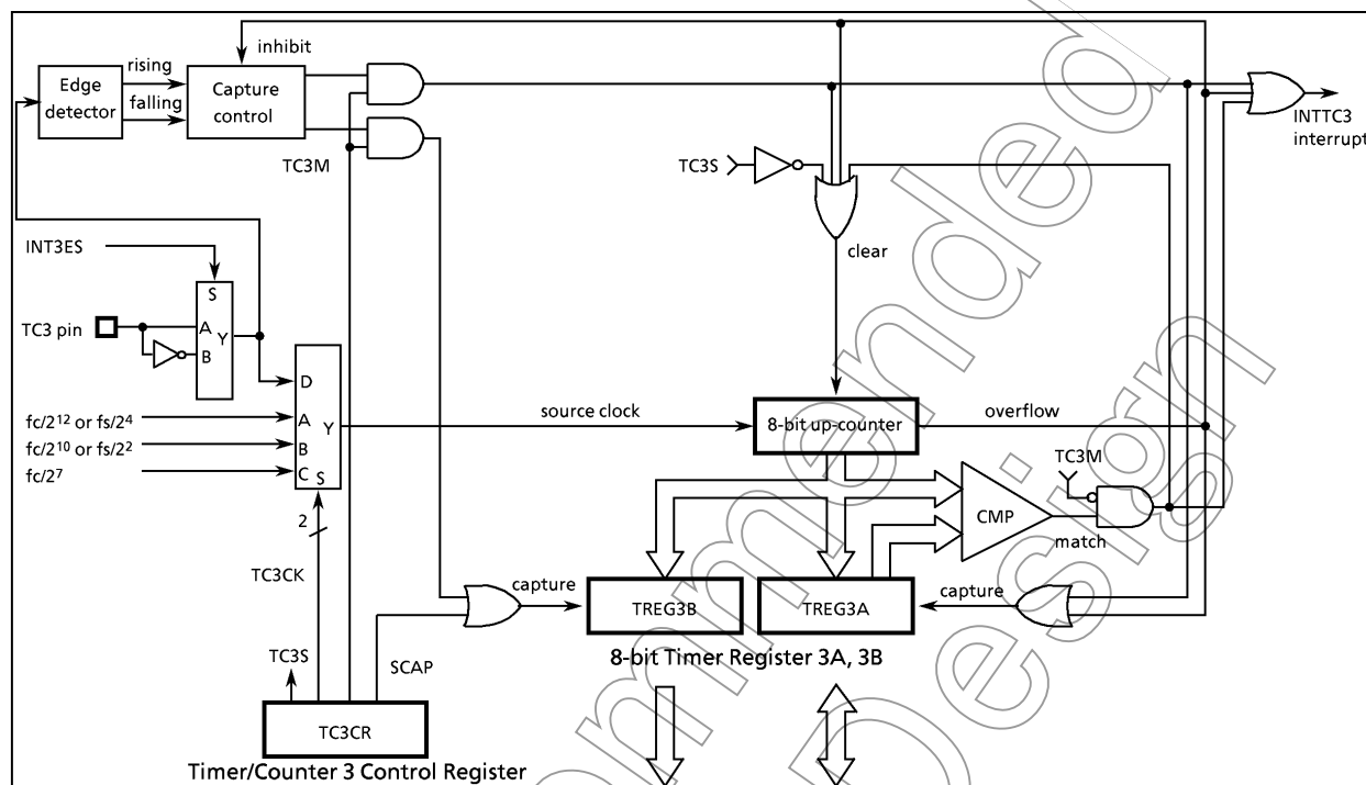
Figure 2-24. Timer/Counter 3
