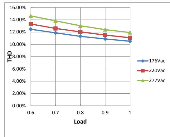
THD Curve
