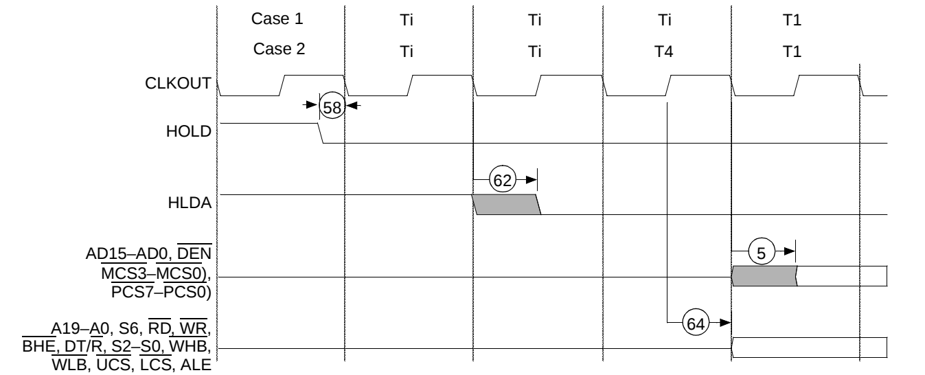
Figure 27. Exiting Bus Hold Waveforms
