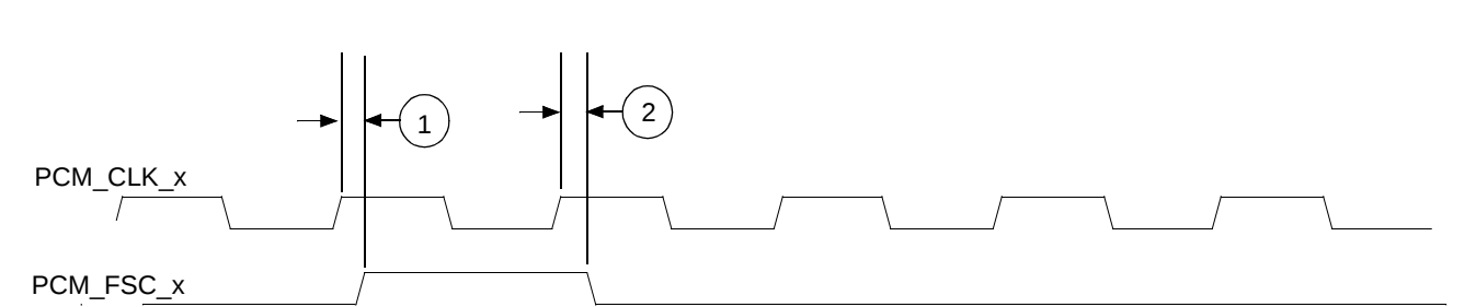
Figure 32. PCM Highway Waveforms (Timing Master)
