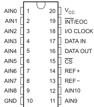
DW or PW Package 20-Pin SOIC or TSSOP Top View
