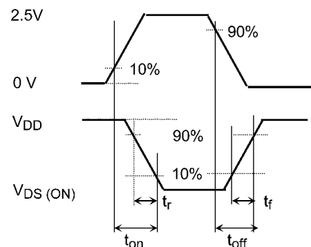
Fig. 7.3.2 Input Waveform/Output Waveform
