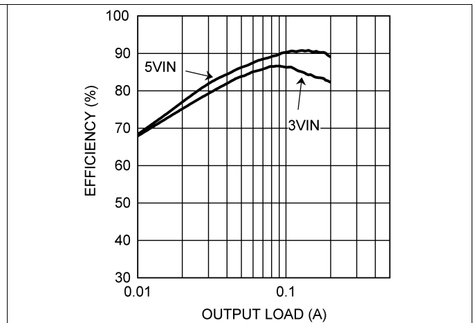
Figure 8. LM2735-Q1Y Efficiency vs Load Current
