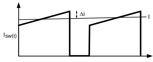
Figure 47. LM2735-Q1 Switch Current
