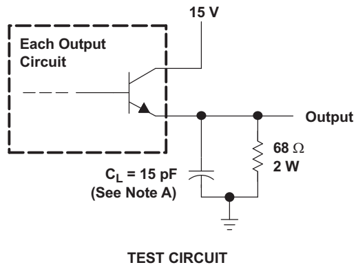
Figure 8. Emitter-Follower Configuration
