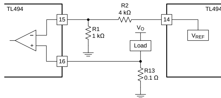
Figure 12. Current-Limiting Circuit
