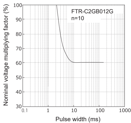
Pulse characteristic
