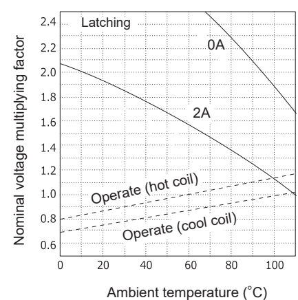
Operate range (latching)
