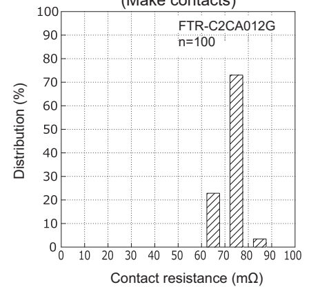
Distribution of contact resistance (Make contacts)
