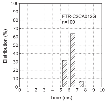
Pulse characteristic
