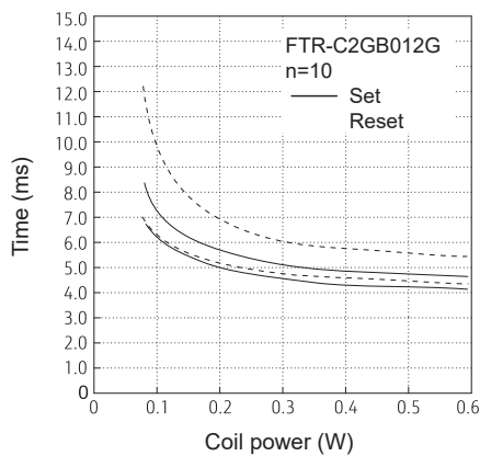
Set/reset time characteristic
