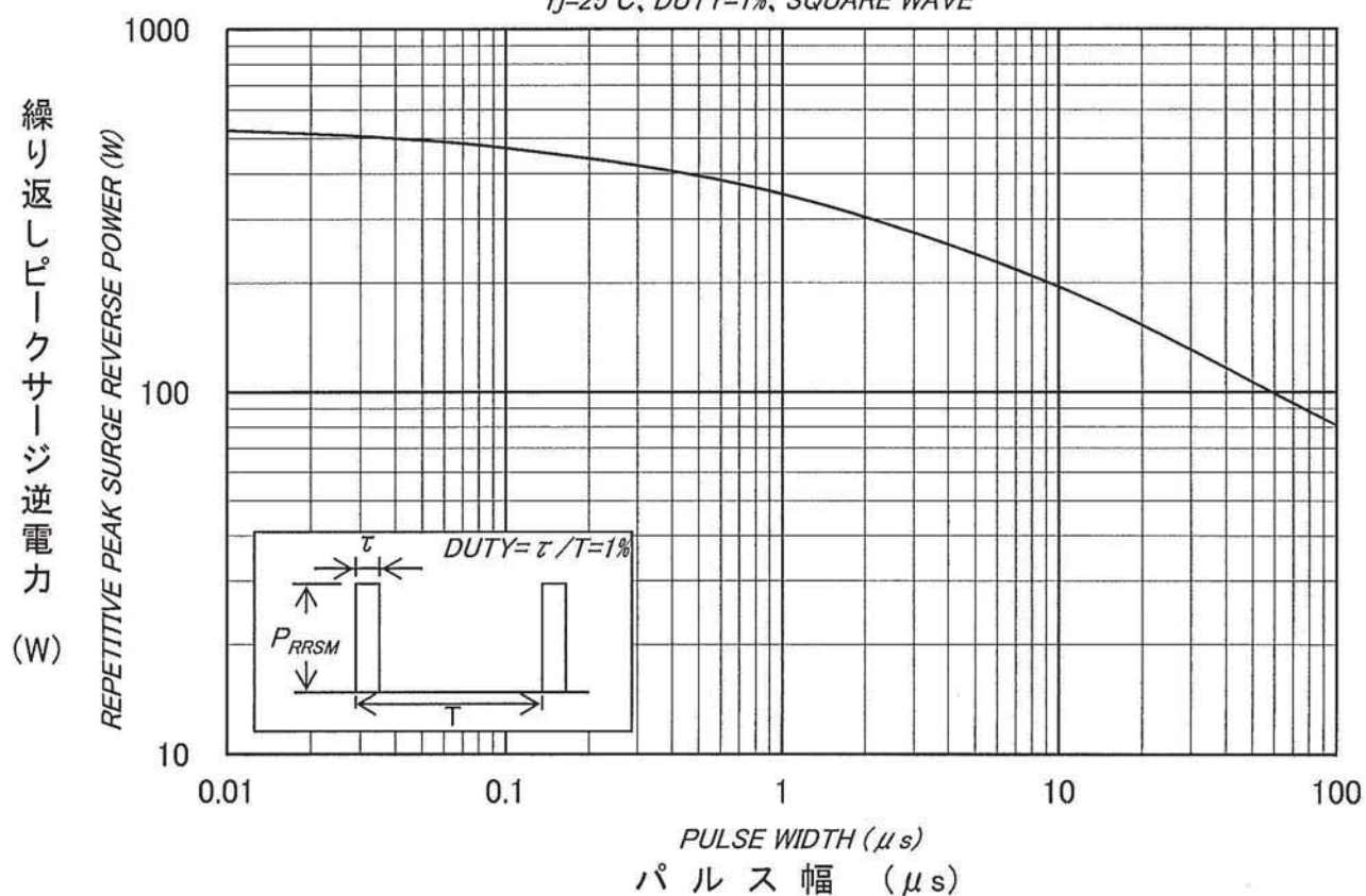
繰り返しピークサージ逆電力定格 REPETITIVE PEAK SURGE REVERSE POWER RATINGS T_J=25^{\circ}\text{C} , DUTY=1%, SQUARE WAVE
