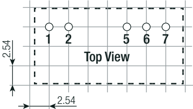
Recommended Footprint Details
