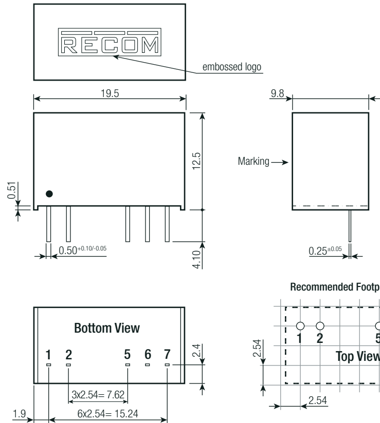
Dimension Drawing (mm)
