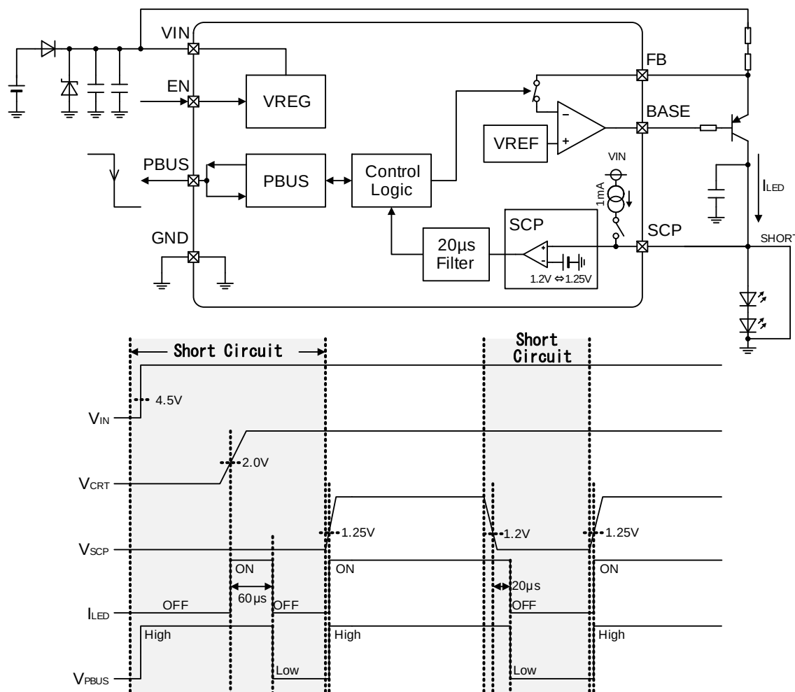
Figure 21. Short Circuit Protection (SCP)
