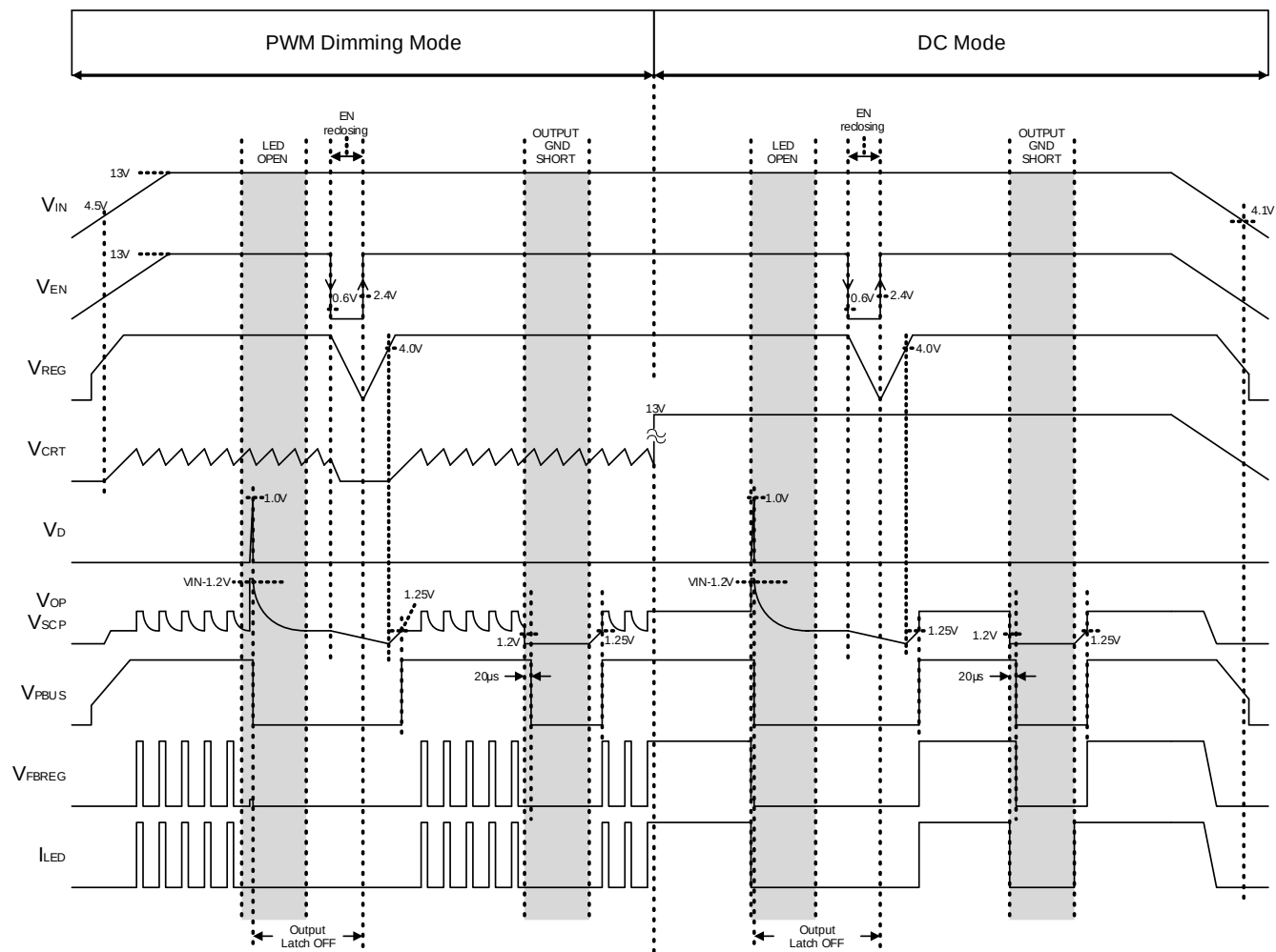
Figure 28. Timing Chart
