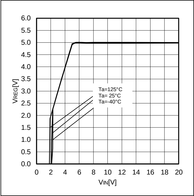
Figure 2. V_{\text{REG}} vs V_{\text{IN}}
