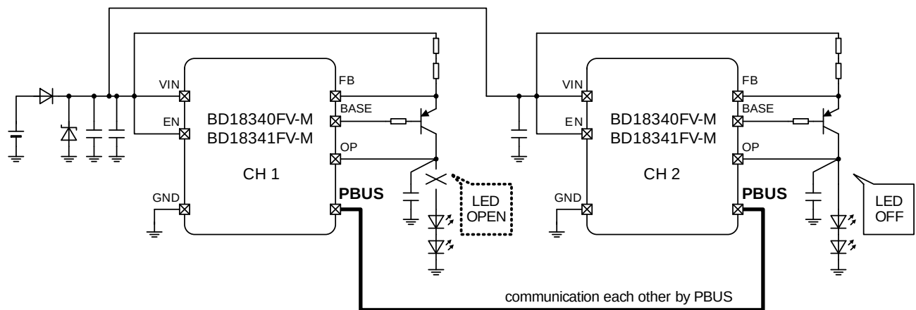
Figure 25. PBUS Function
