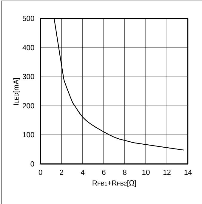
Figure 4. I_{\text{LED}} vs R_{\text{FB1}} + R_{\text{FB2}}
