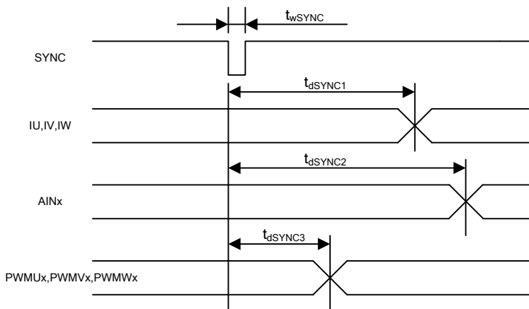
Figure 5 SYNC timing
