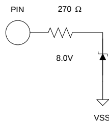
Figure 20 VPP programming pin I/O structure
