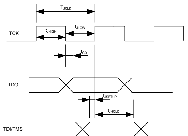
Figure 15 JTAG timing
