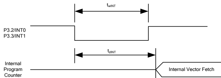
Figure 8 Interrupt timing
