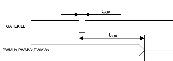
Figure 6 Gatekill timing
