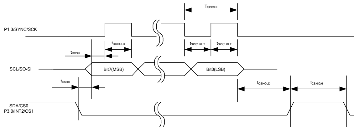
Figure 11 SPI read timing
