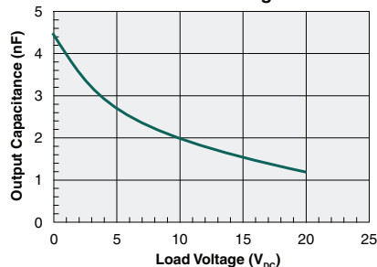
Typical Output Capacitance vs. Load Voltage
