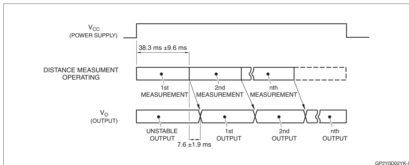
Figure 3. Timing Diagram
