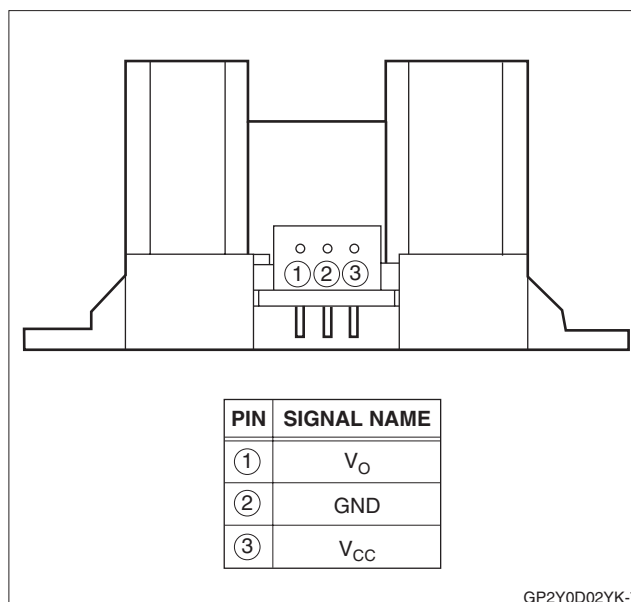
Figure 1. Pinout
