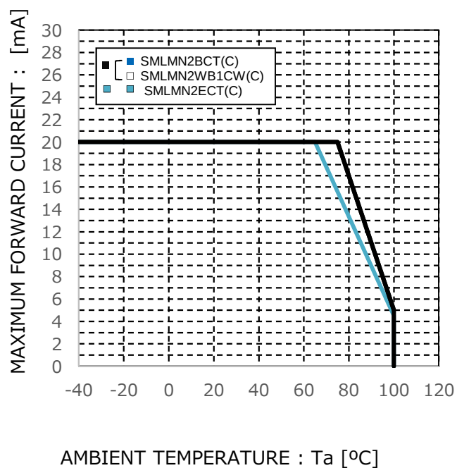
Fig.4 Derating
