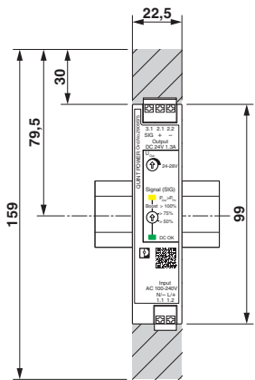
Dimensional drawing
