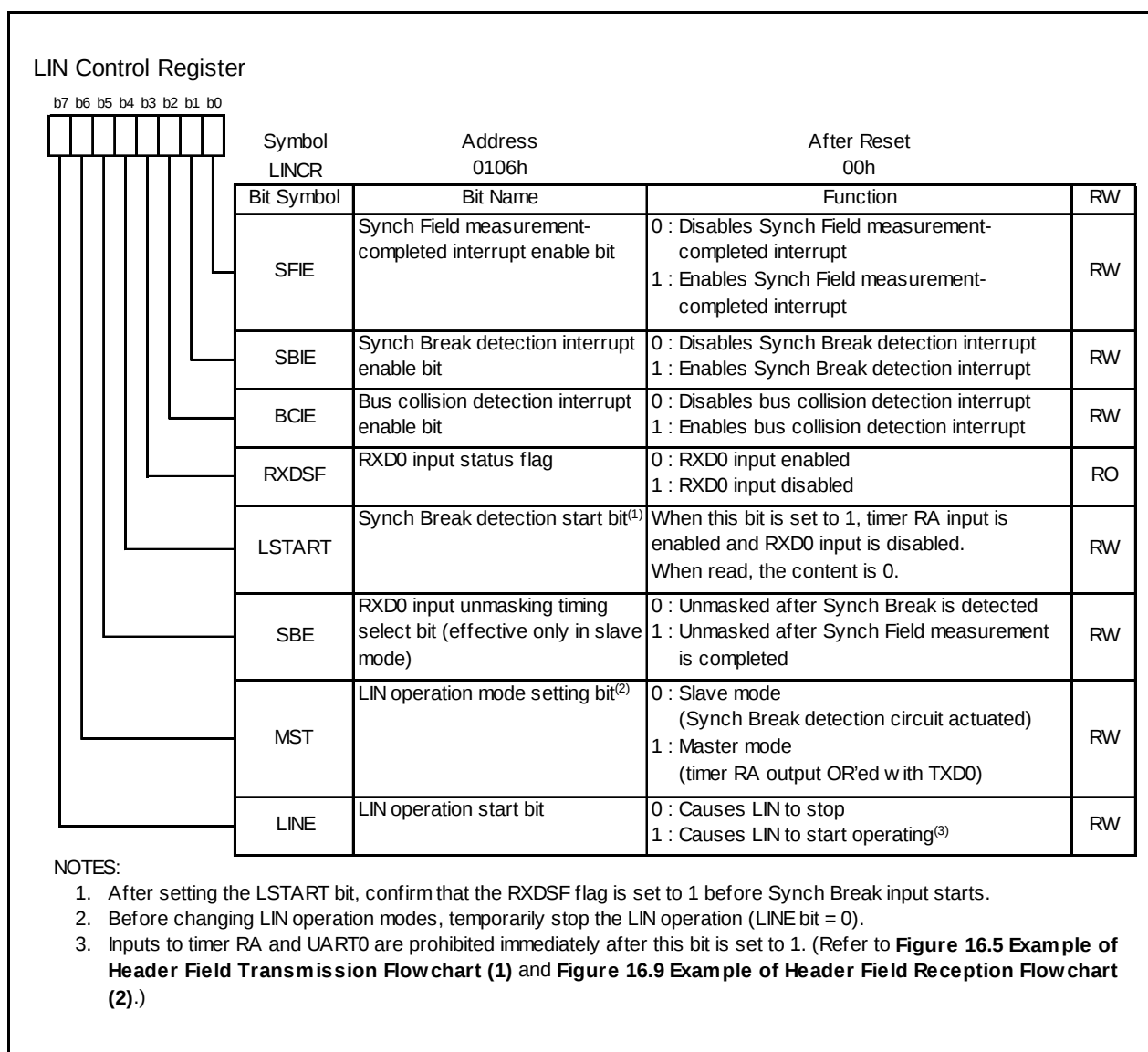
Figure 16.2 LINCX Register
