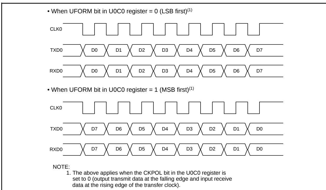
Figure 15.10 Transfer Format
