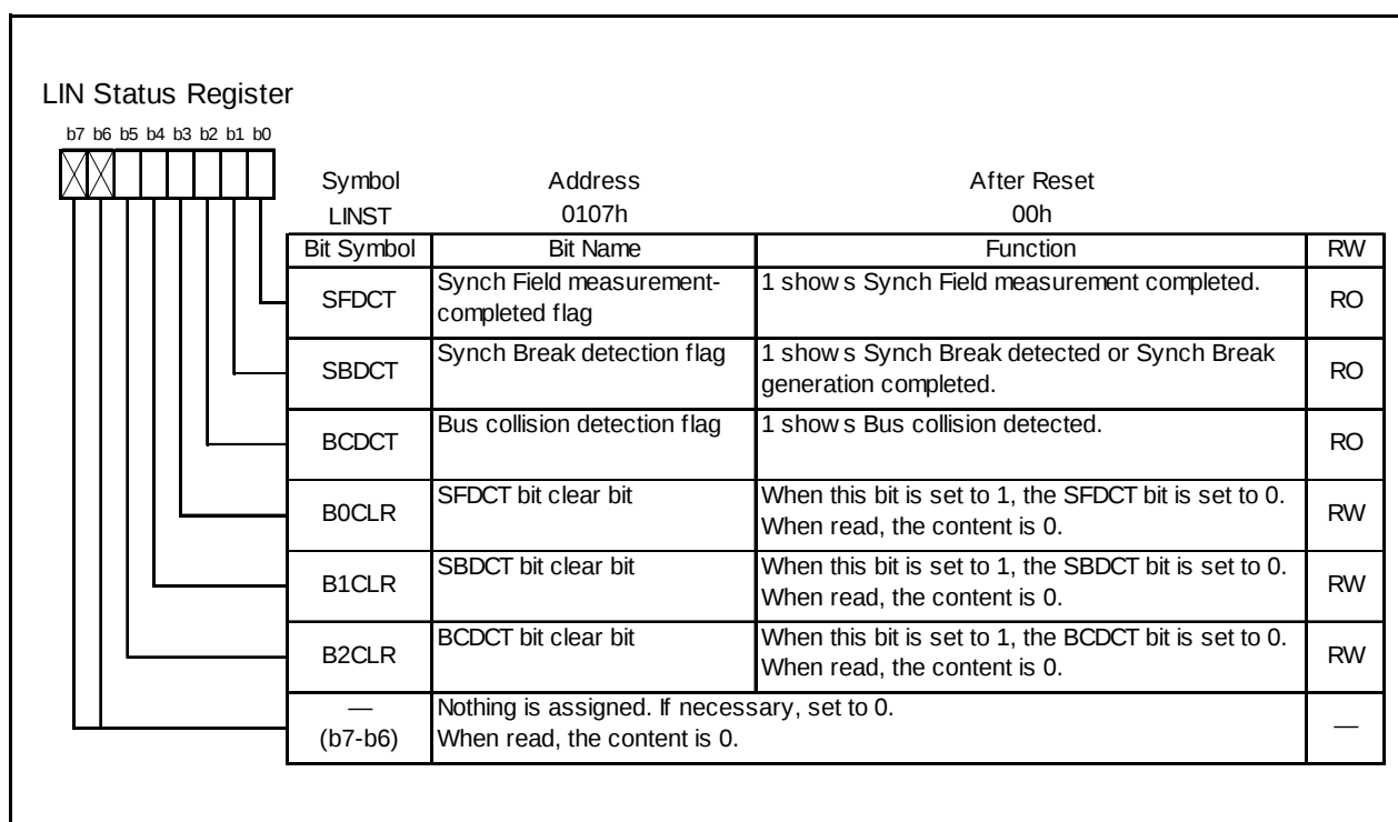
Figure 16.3 LINST Register
