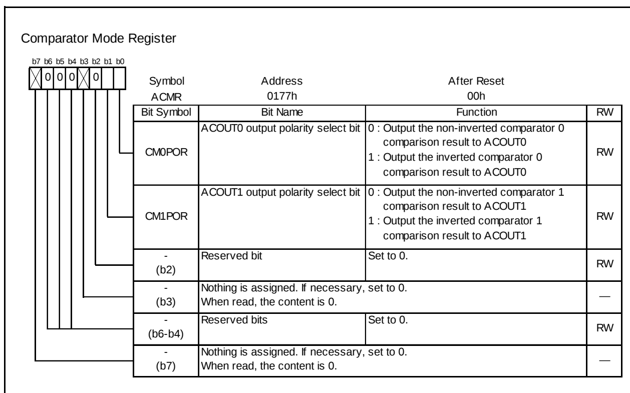
Figure 19.3 ACMR Register
