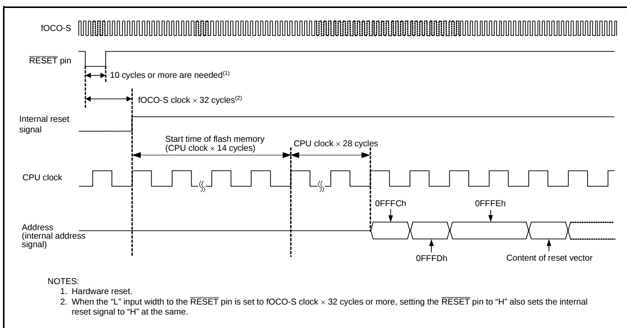
Figure 5.3 Reset Sequence
