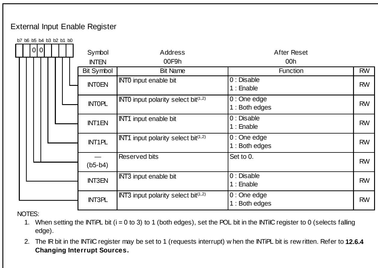
Figure 12.12 \text{INTEN} Register
