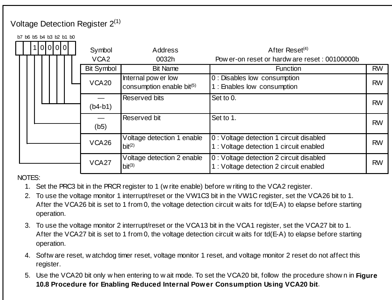
Figure 10.7 VCA2 Register
