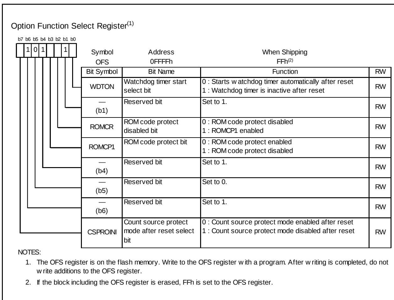
Figure 20.4 OFS Register
