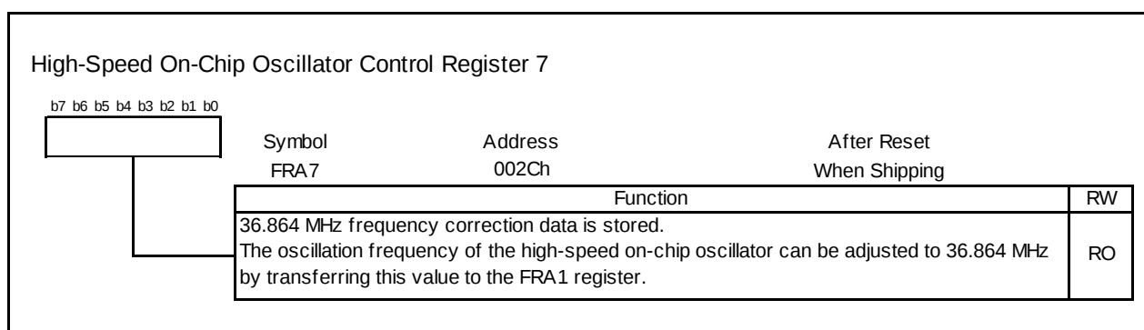
Figure 10.6 FRA7 Register
