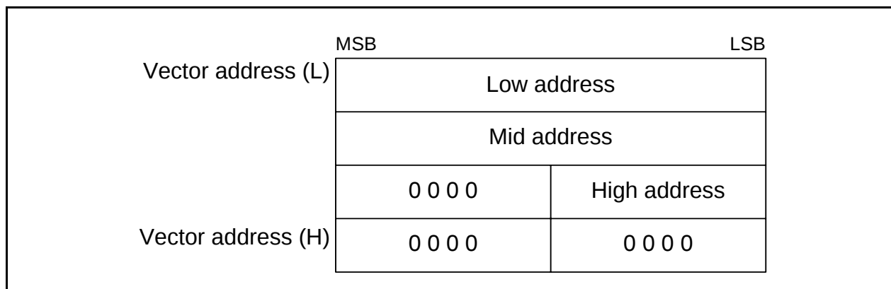
Figure 12.2 Interrupt Vector
