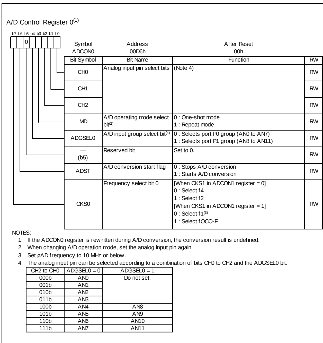
Figure 17.2 ADCON0 Register
