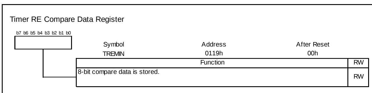
Figure 14.63 TREMIN Register in Output Compare Mode
