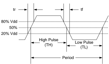
Figure 3. Waveform [6]
