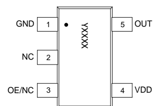
Figure 1. Pin Assignments
