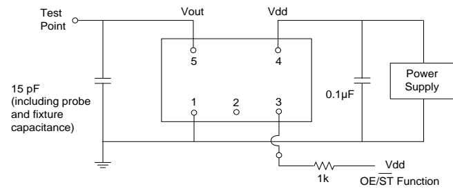
Figure 2. Test Circuit [6]
