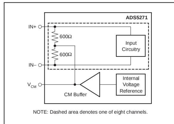
Figure 15. Analog Input Bias Circuitry
