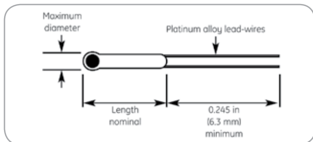
NTC Types P20/25/30 dimensions
