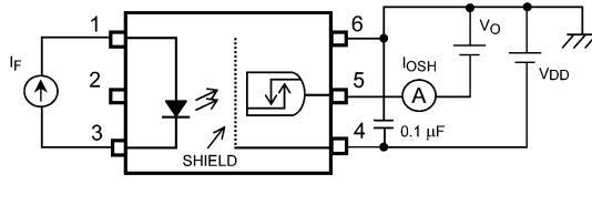
Fig. 12.1.6 IOSH Test Circuit
