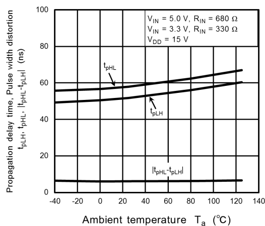
Fig. 12.2.13 t_{PLH} , t_{PHL} , |t_{PHL} - t_{PLH}| - T_a
