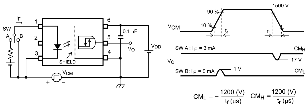
Fig. 12.1.8 Common-Mode Transient Immunity Test Circuit and Waveform
