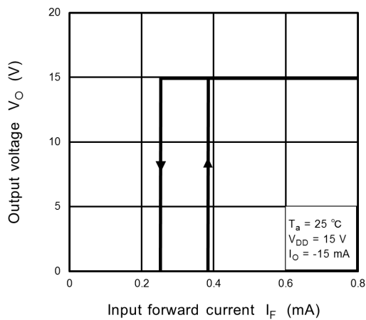
Fig. 12.2.4 V_O - I_F(IHYS)
