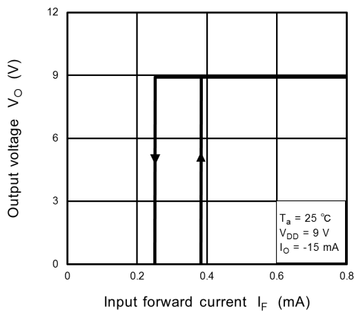
Fig. 12.2.3 V_O - I_F(IHYS)
