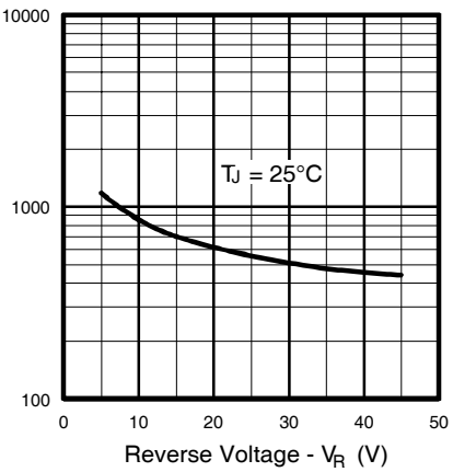
Fig. 3 - Typical Junction Capacitance Vs. Reverse Voltage (Per Leg)
