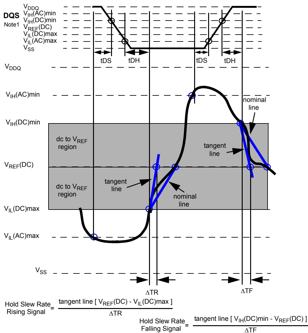
Figure 14. Illustration of tangent line for tDH (single-ended DQS)
