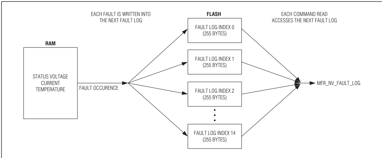
Figure 2. MFR_NV_FAULT_LOG
