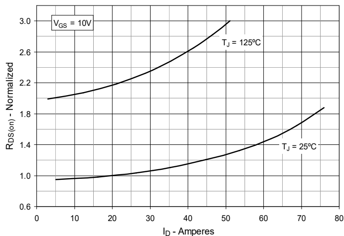
Fig. 5. R_{DS(on)} Normalized to I_D = 21\text{A} Value vs. Drain Current
