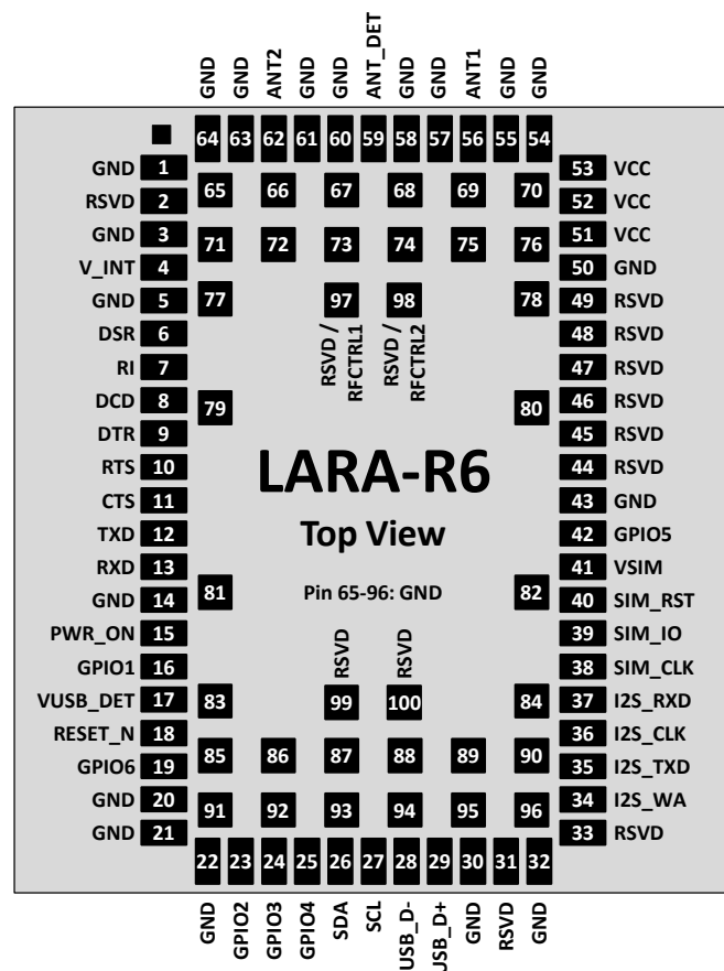
Figure 2: LARA-R6 series pin assignment (top view)
