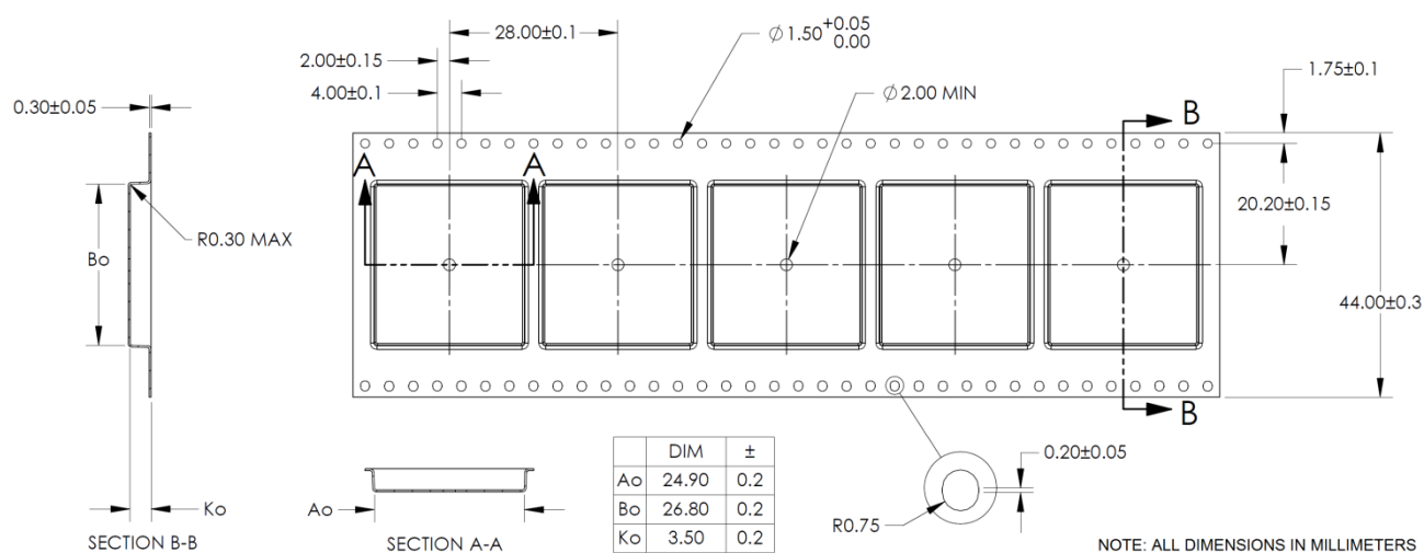
Figure 7: LARA-R6 series modules tape dimensions
