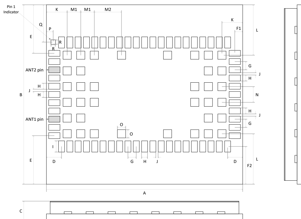
Figure 5: LARA-R6 series dimensions (bottom and side views)
