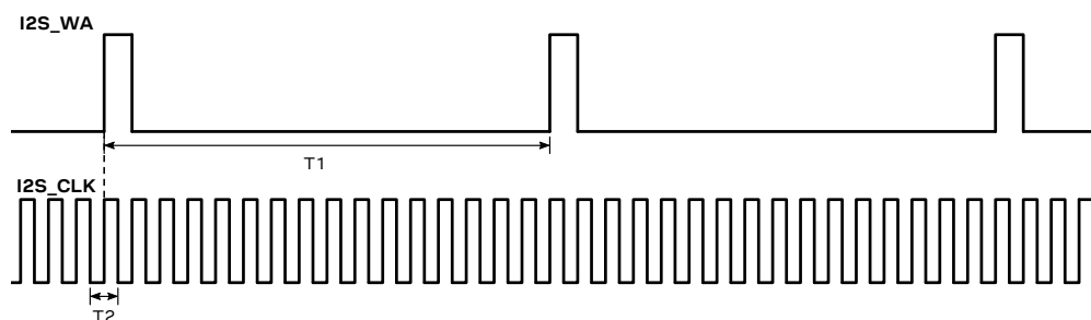
Figure 4: AC characteristics of digital audio interface in PCM mode (short synchronization signal), host role
