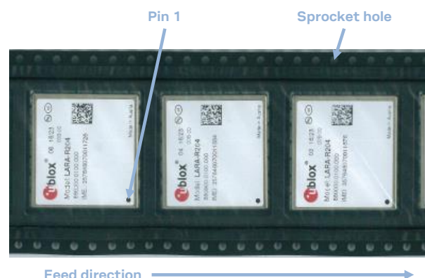
Figure 6: Orientation for LARA modules on tape
