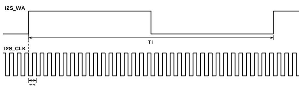
Figure 3: AC characteristics of digital audio interface in Normal I2S mode (long synchronization signal), host role
