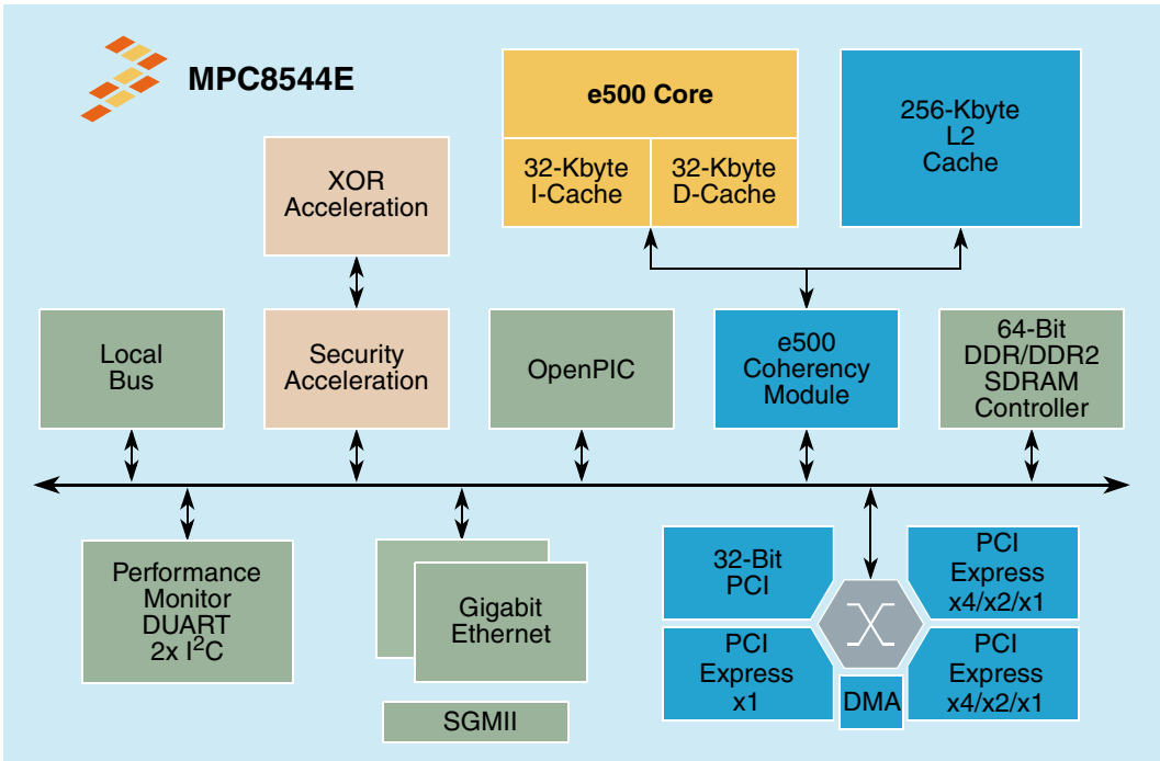
Figure 1. MPC8544E Block Diagram
