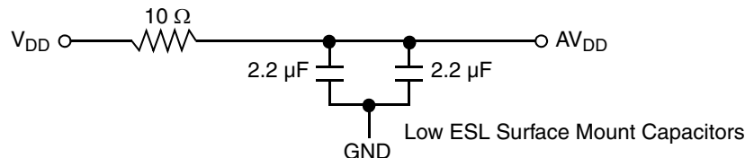
Figure 65. MPC8544E PLL Power Supply Filter Circuit
