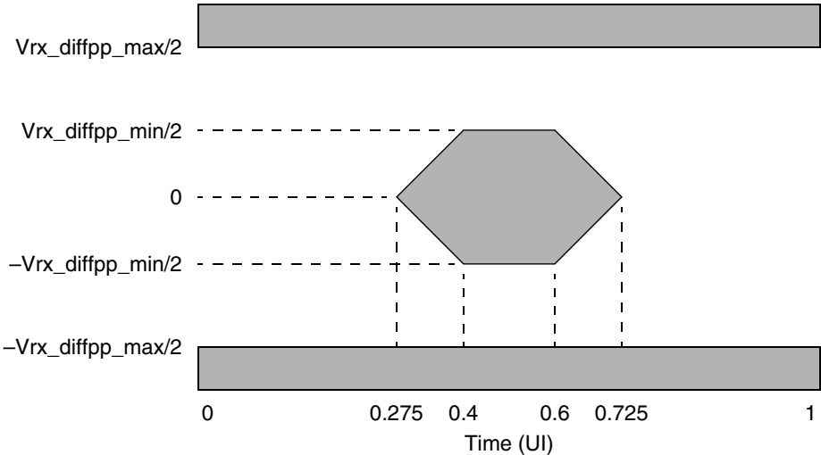
Figure 9. Receive Input Compliance Mask
