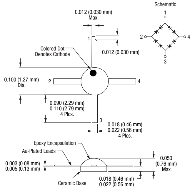
Figure 21. -257 Package Dimensions
