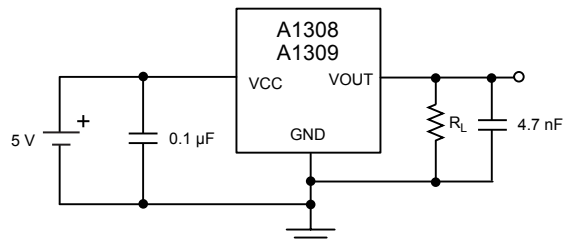
Figure 6: Typical Application Circuit
