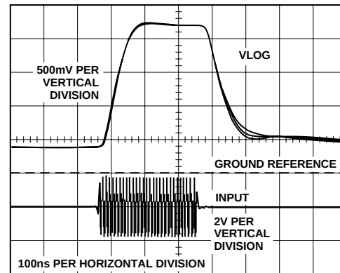
Figure 5. Large Signal RSSI Pulse Response with R_L = 100\text{ }\Omega and C_L = 33\text{ pF} , 100\text{ pF} and 330\text{ pF} (Overlapping Curves)
