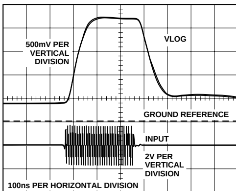
Figure 3. Large Signal RSSI Pulse Response with C_L = 100\text{ pF} and R_L = 50\text{ }\Omega and 75\text{ }\Omega (Curves Overlap)
