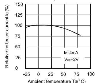
Fig. 4 Relative Collector Current vs. Ambient Temperature
