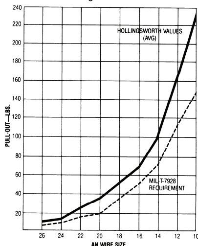
CHART 9074 Tensile Strength Test 26-10 AWG
