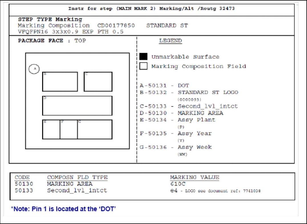
Figure 17. Marking specifications
