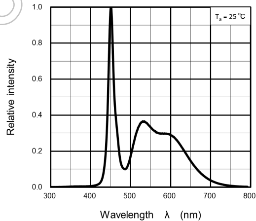
Fig. 8.6 Wavelength Characteristic
