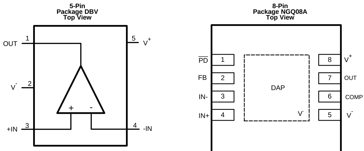
Pin Functions
