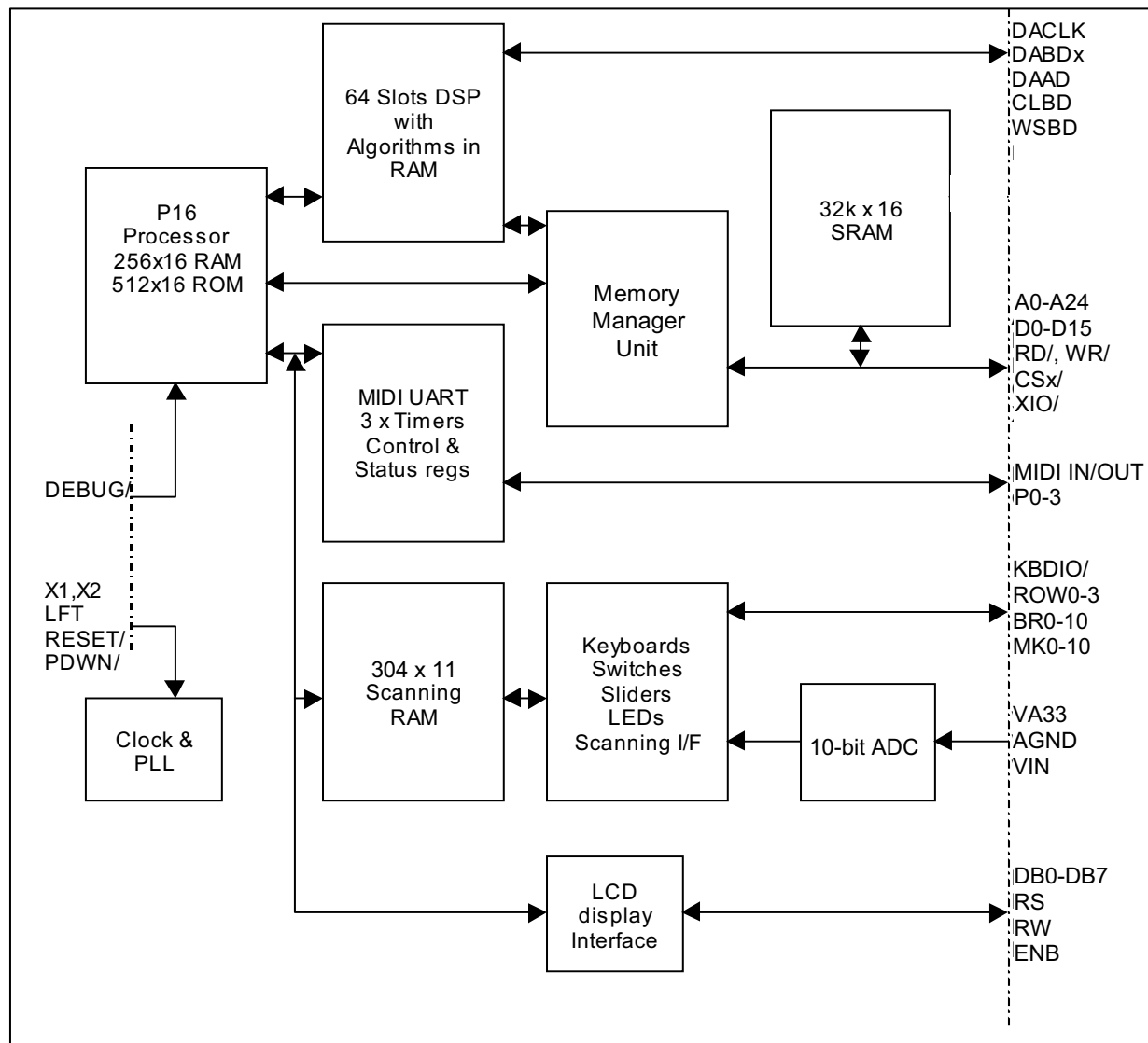
Figure 3-1. Internal Architecture
