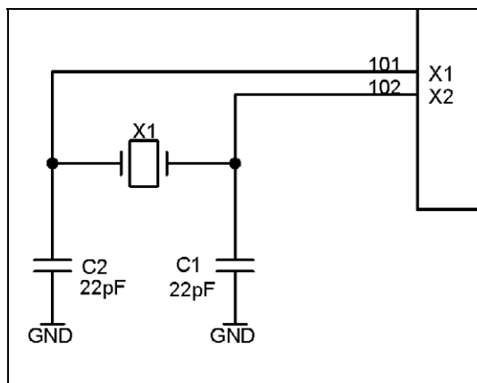
Figure 9-1. Recommend Crystal Compensation
