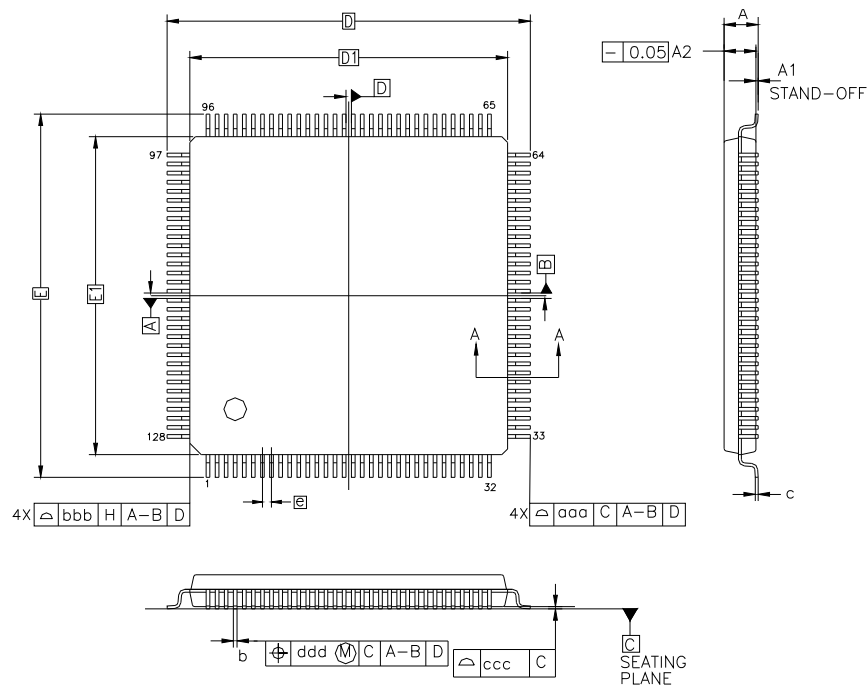
Figure 6-1. Mechanical Dimensions
