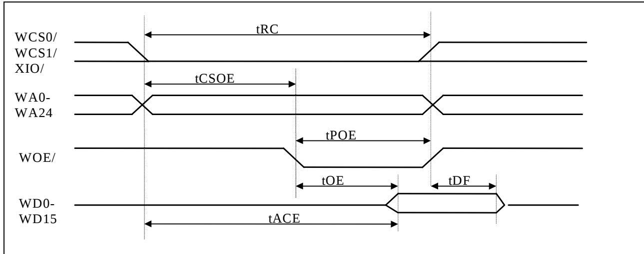
Figure 8-2. External ROM/Flash, RAM, I/O Read Timing
