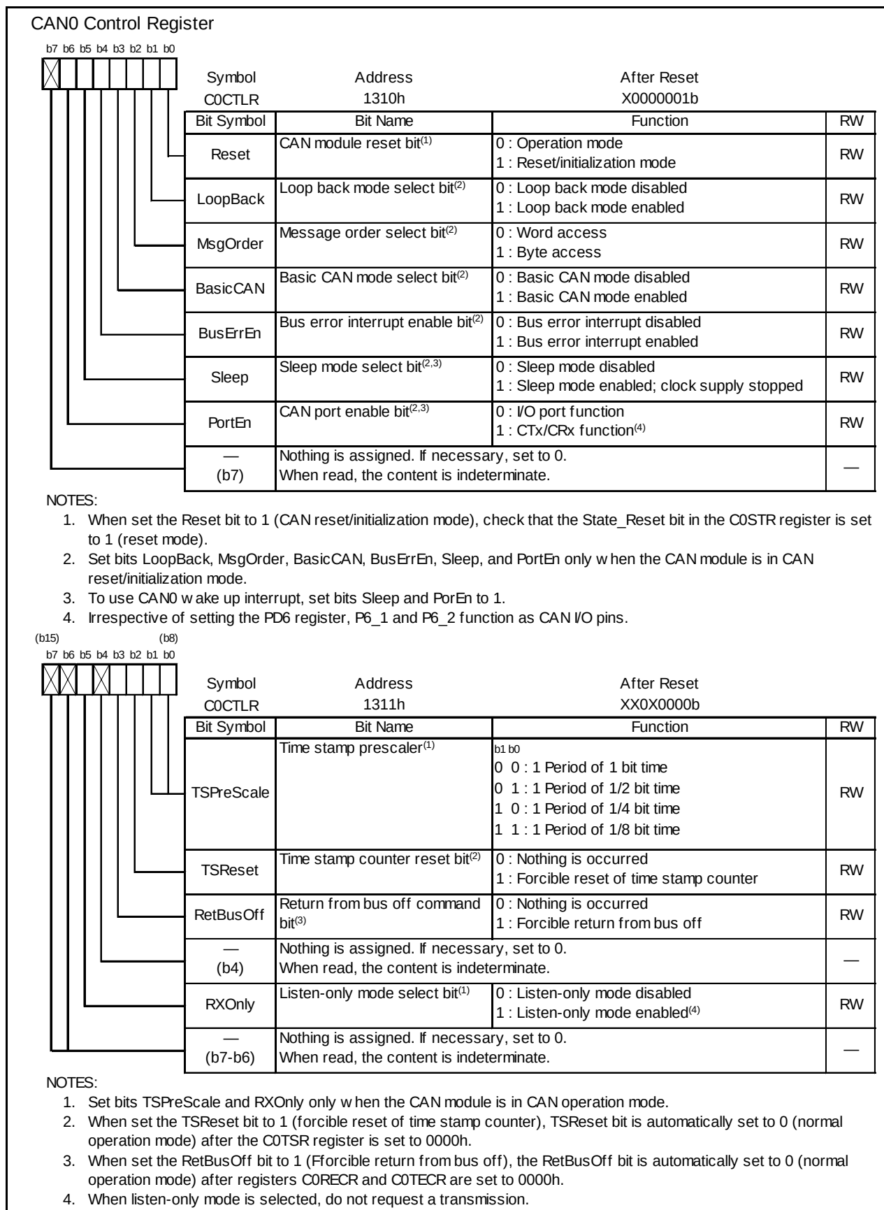
Figure 18.7 C0CTLR Register
