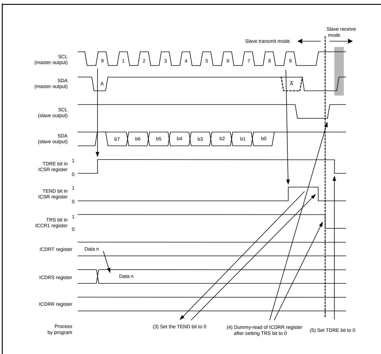
Figure 16.38 Operating Timing in Slave Transmit Mode (I²C Bus Interface Mode) (2)
