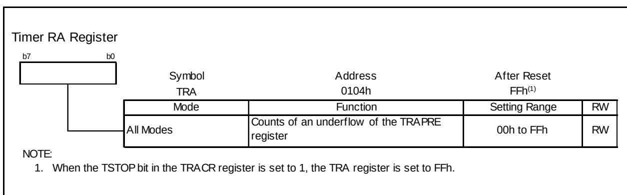
Figure 14.4 TRA Register
