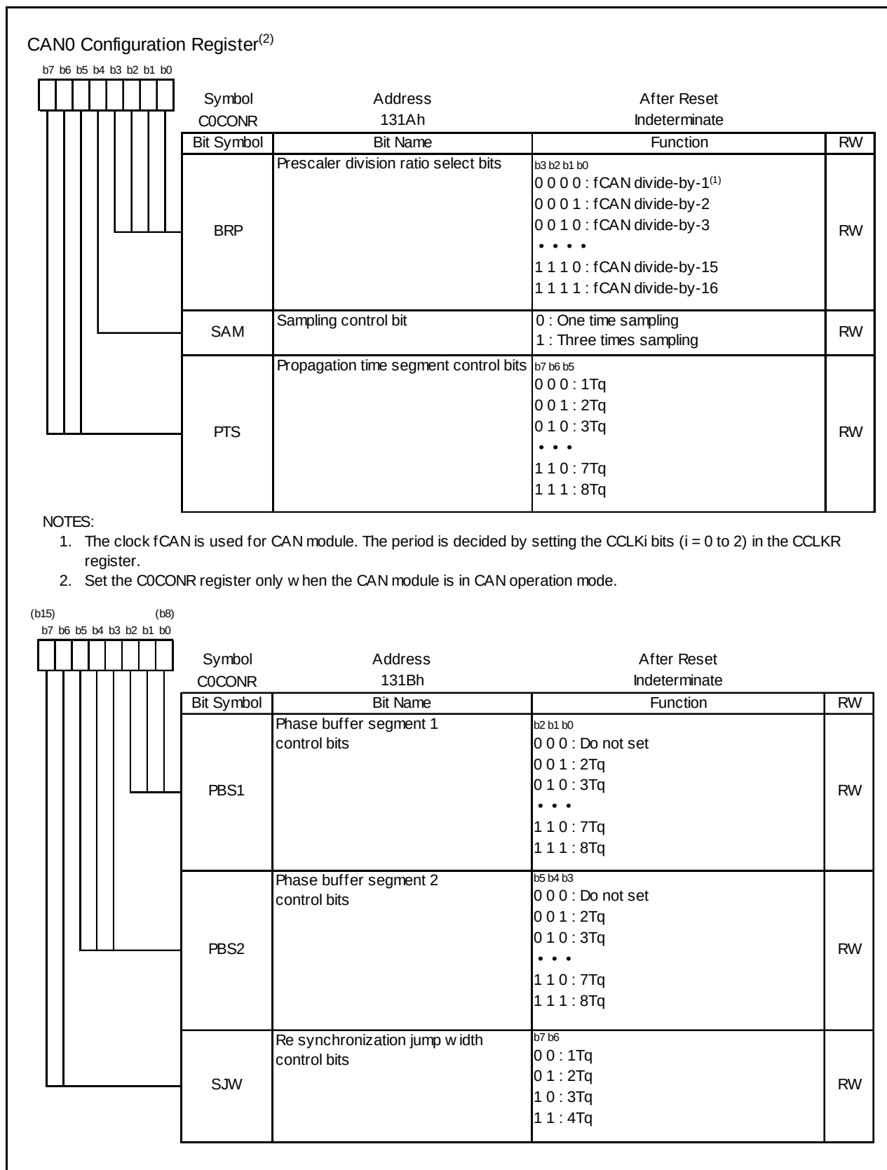
Figure 18.12 C0CONR Register
