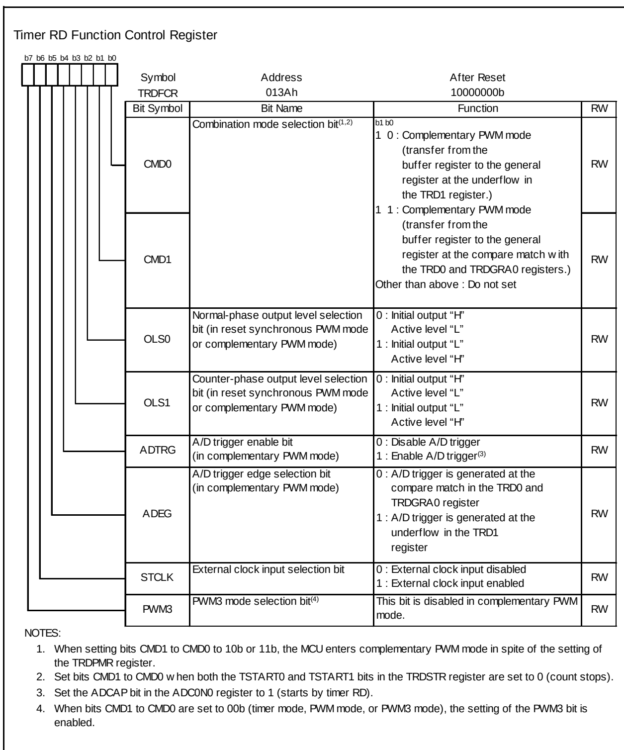
Figure 14.89 TRDFCR Register in Complementary PWM Mode
