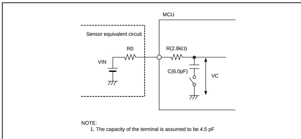
Figure 19.11 Analog Input Pin and External Sensor Equivalent Circuit
