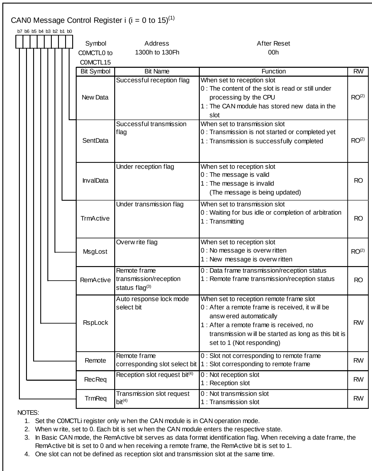
Figure 18.6 C0MCTLi Register
