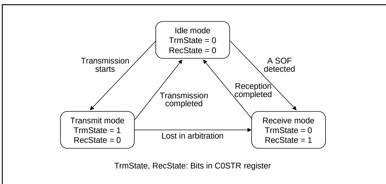
Figure 18.17 Sub Modes in CAN Operation Mode
