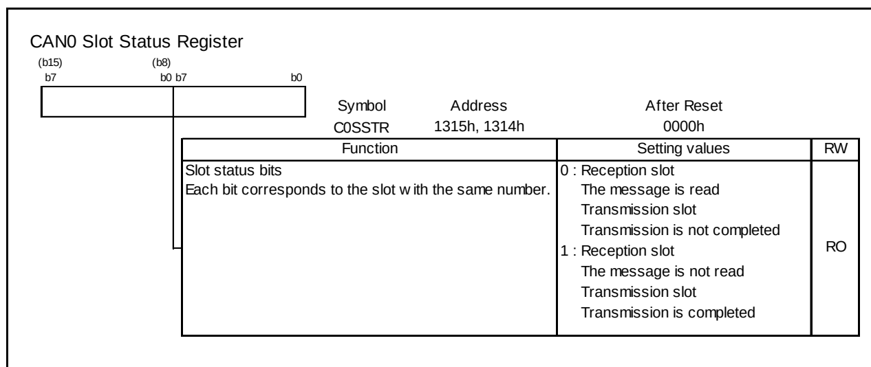
Figure 18.9 C0SSTR Register
