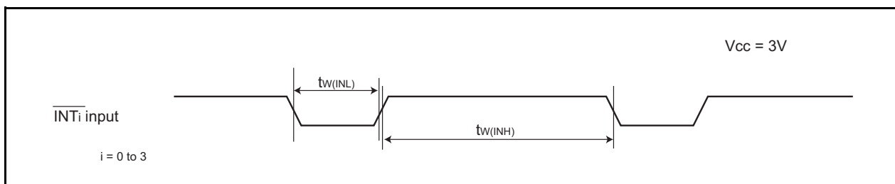
Figure 21.15 External Interrupt \overline{INTi} Input Timing Diagram when Vcc = 3 V (i = 0 to 3)
