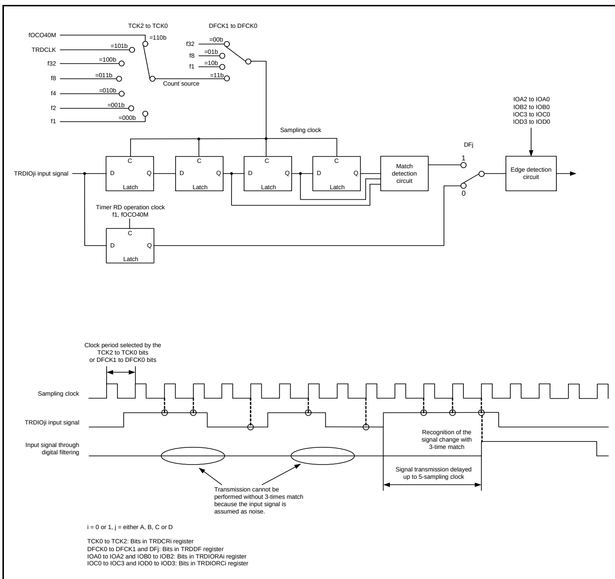
Figure 14.46 Block Diagram of Digital Filter
