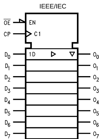
Figure 1. Logic Symbol
