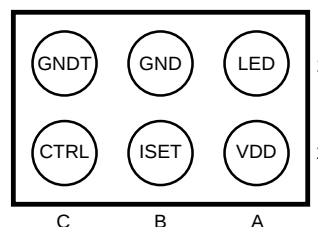
Figure 2. Bottom View
