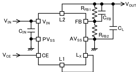
< Typical application circuits Type F>
