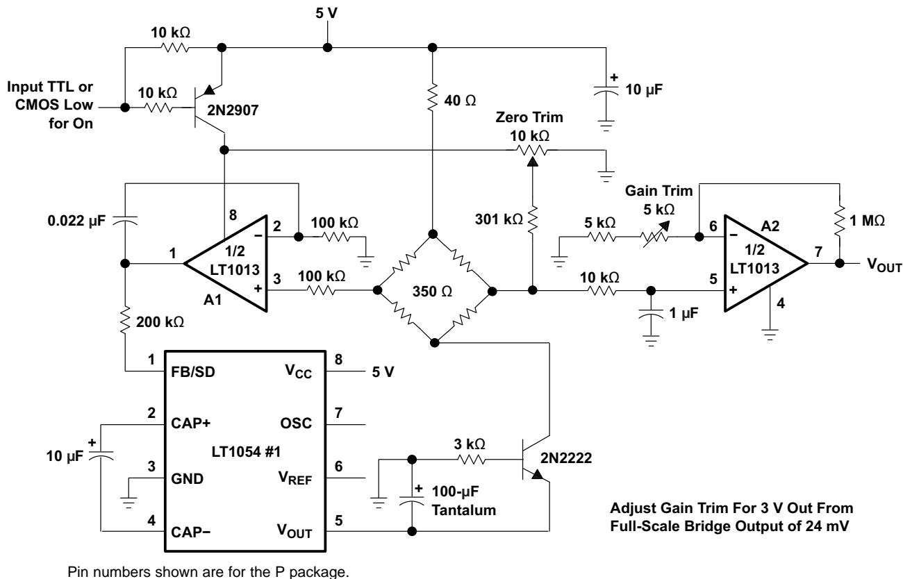
Figure 24. Strain-Gage Bridge Signal Conditioner
