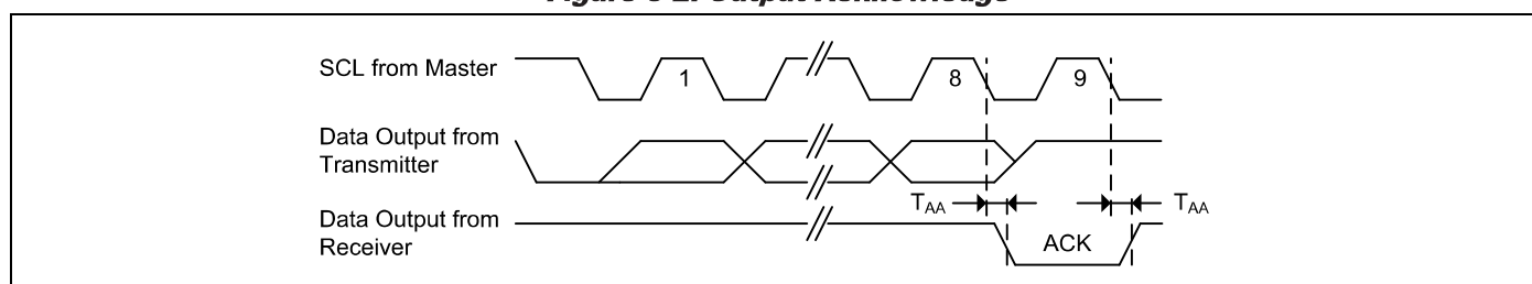
Figure 5-2. Output Acknowledge
