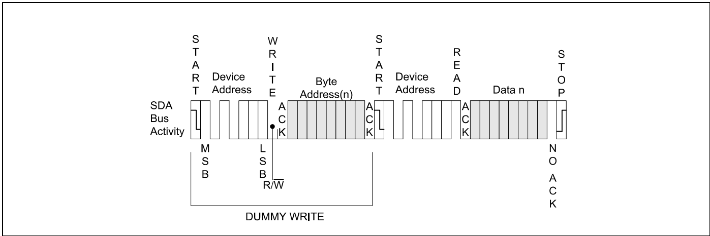
Figure 5-9. Random Address Read
