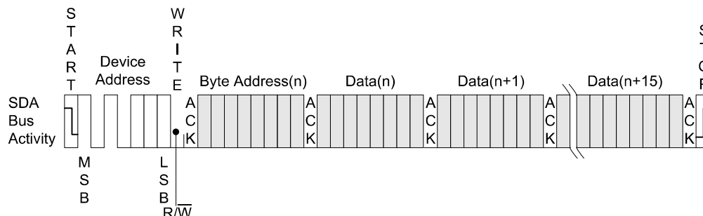
Figure 5-7. Page Write
