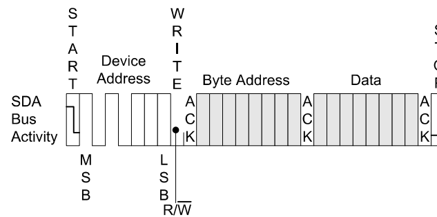
Figure 5-6. Byte Write
